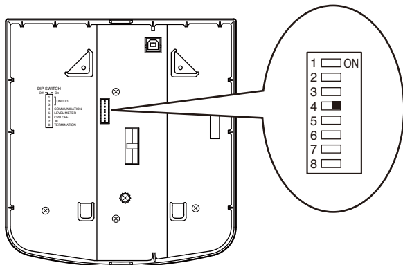
RM-200SF bottom
