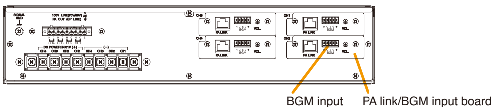
Amplifier's rear
