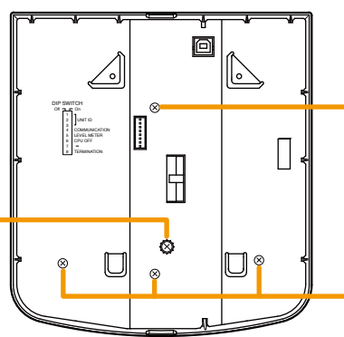
RM-200SF bottom
